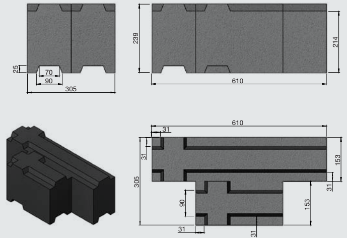
Corner Ballistic Block B (34kg)
