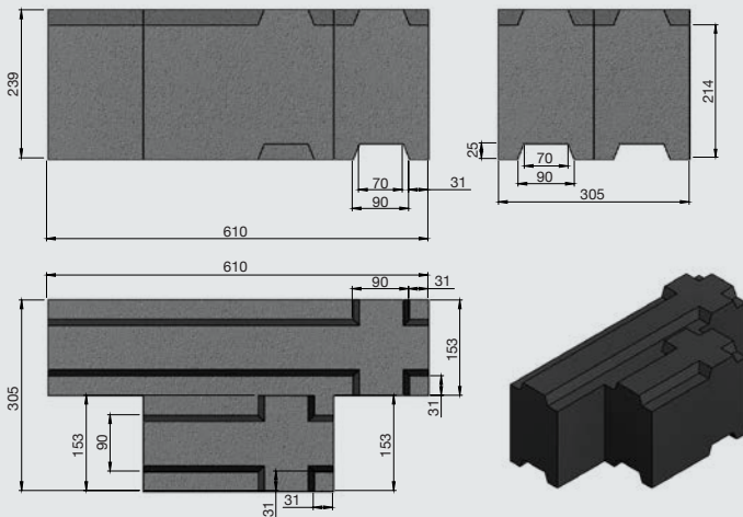
Corner Ballistic Block A (34kg)
