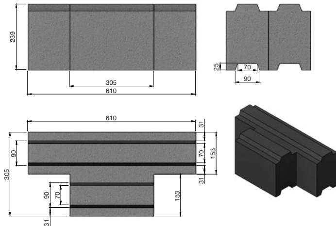
Standard Ballistic Block (34kg)
