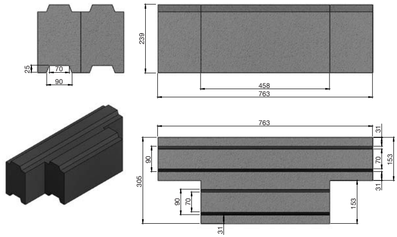
Large Ballistic Block (47kg)
